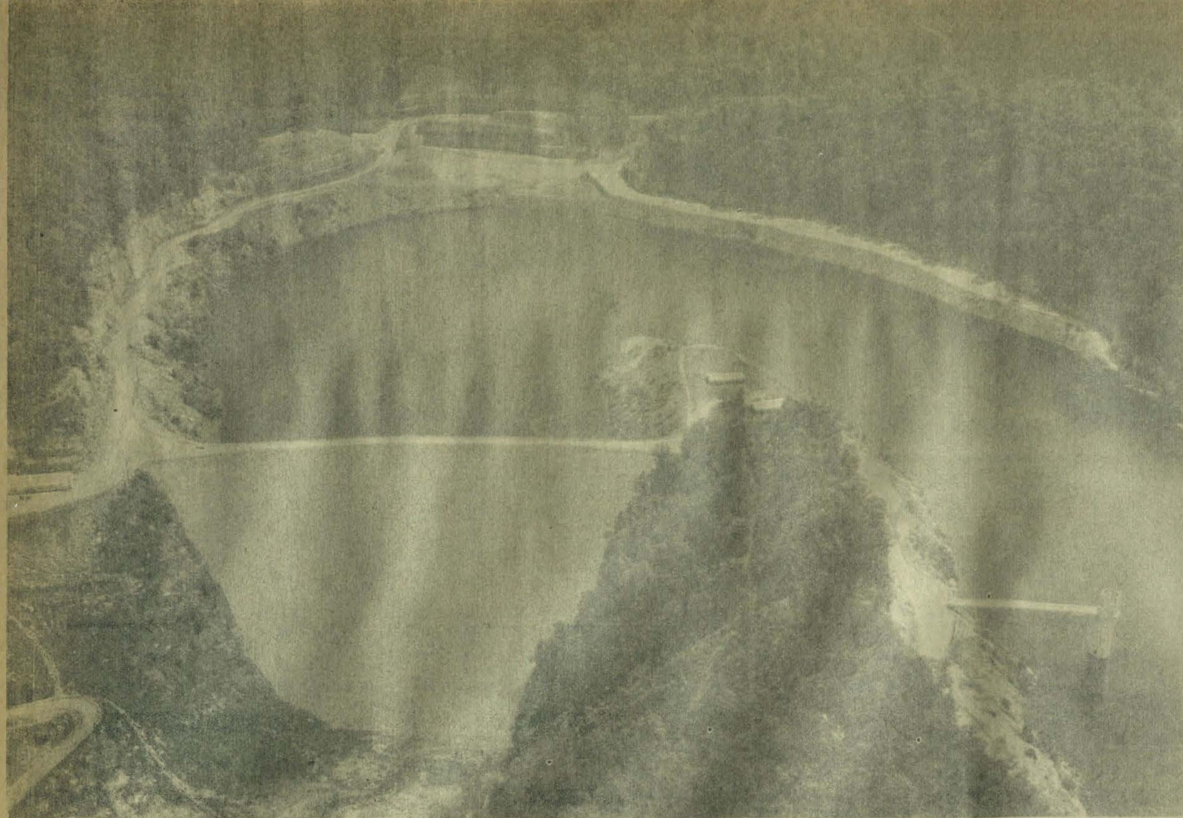
THE DAM THAT PAID FOR ITSELF BEFORE IT WAS COMPLETED. John Flanagan Dam, near Haysi, Va., was credited with saving Prestonsburg and other Big Sandy towns from $15.4 million damages in the 1963 flood.
