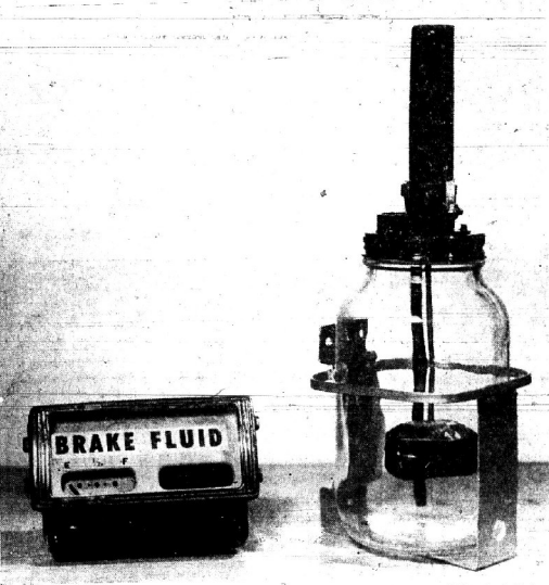
Auxiliary fluid container devised by Prestonsburg men is shown at right. At left is dashboard gauge which is devised to keep driver aware of brakes condition at all times.
