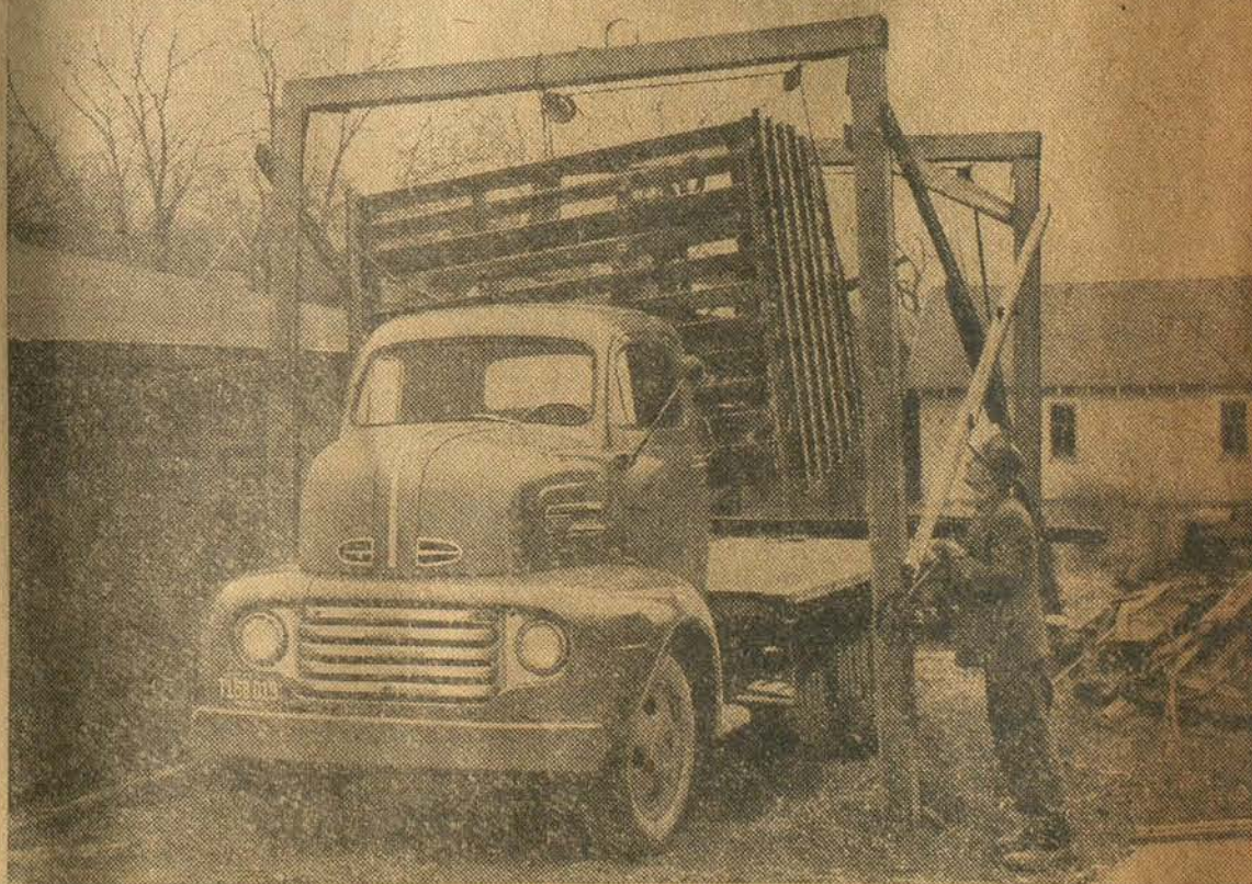
John J. Schaffer, livestock hauler out of Cedar Lake, designed this mechanism which permits him to change bodies on his new Ford Bonus Built Truck, in double-quick time, and all by himself.
